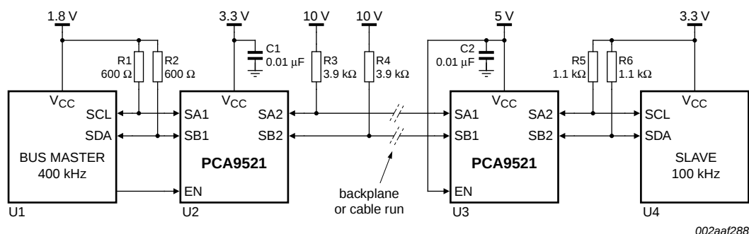
Fig 11. PCA9521 typical buffer application
