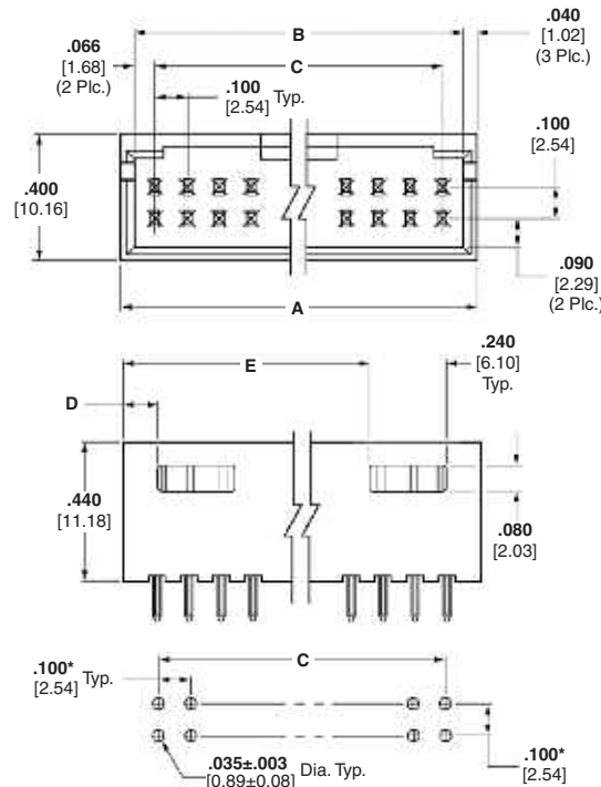
Recommended PC Board Hole Layout (for .055 [1.40] min. thick PC board)
