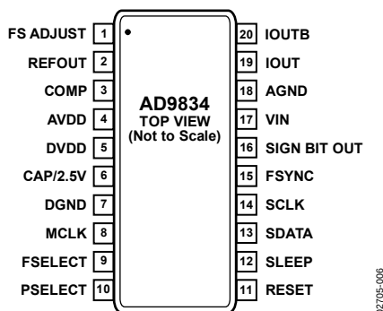
Figure 6. Pin Configuration
