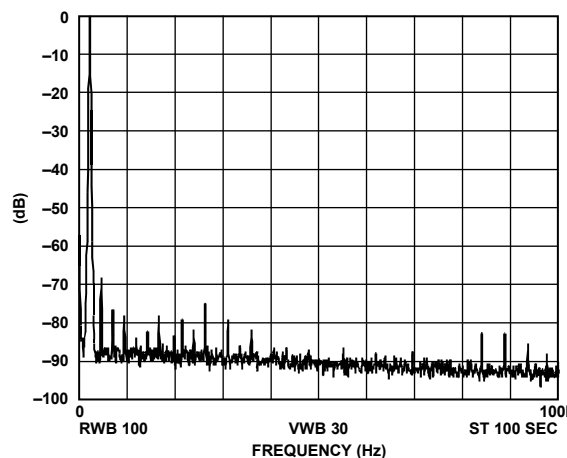
Figure 18. f_{MCLK} = 10 \text{ MHz} ; f_{OUT} = 2.4 \text{ kHz} , Frequency Word = 000FBA9
