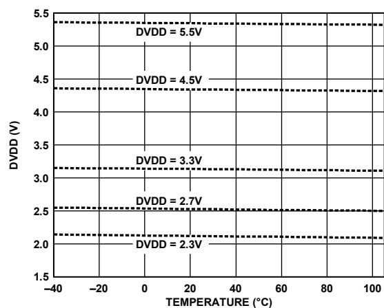
Figure 17. SIGN BIT OUT High Level, I_{SINK} = 1 \text{ mA}
