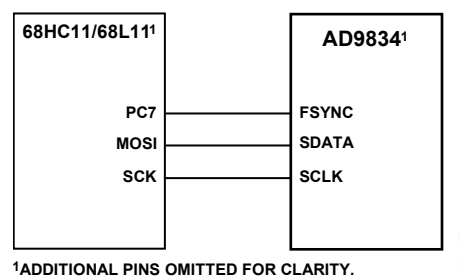
Figure 36. 68HC11/68L11 to AD9834 Interface
