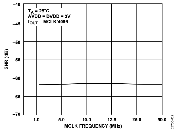
Figure 12. SNR vs. MCLK Frequency
