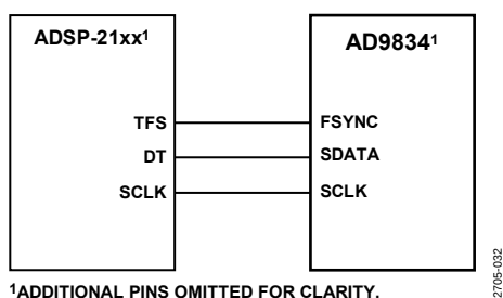
Figure 35. ADSP-21xx to AD9834 Interface
