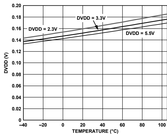
Figure 16. SIGN BIT OUT Low Level, I_{SINK} = 1 \text{ mA}
