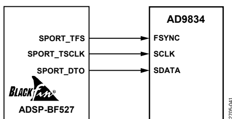
Figure 39. SDP to AD9834 Interface
