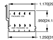
MARKING DETAIL FRONT VIEW VCH CONNECTOR HOUSING
