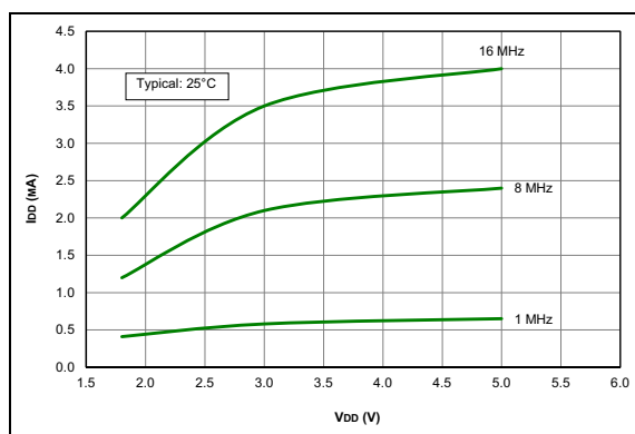
FIGURE 28-17: I_{DD} Typical, HFINTOSC Mode, PIC18F1XK50 Only.
