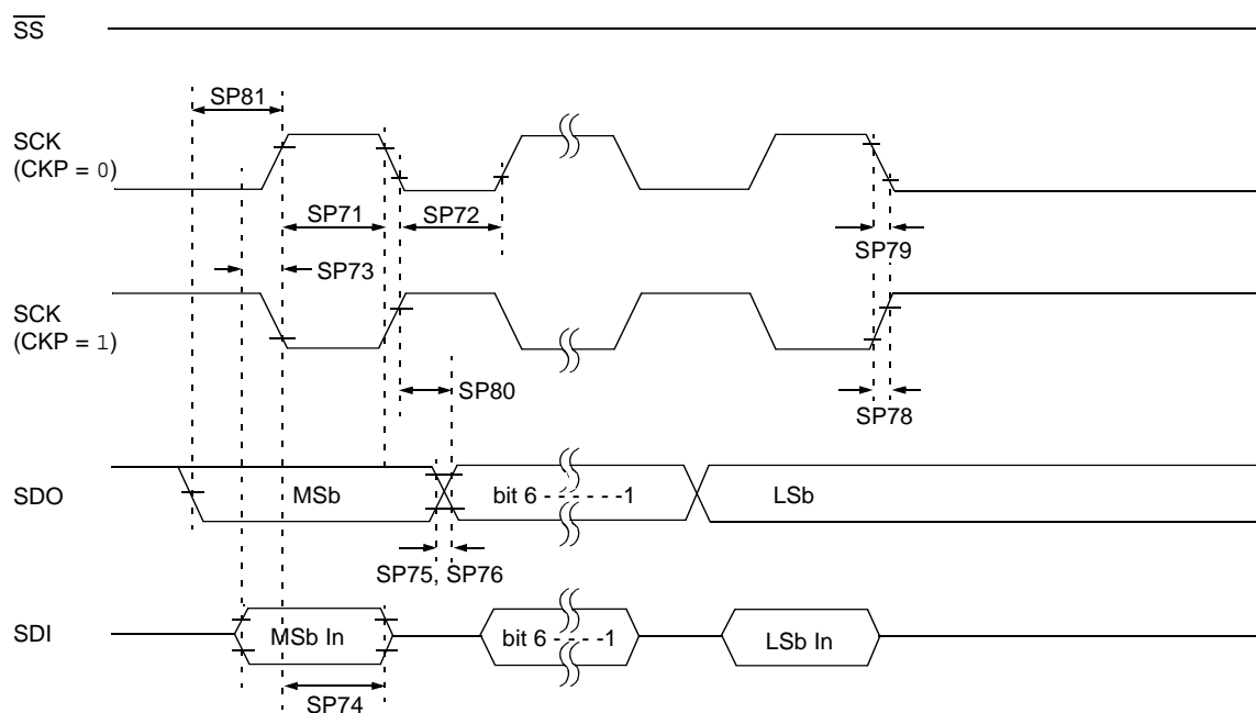
FIGURE 27-16: SPI MASTER MODE TIMING (CKE = 1, SMP = 1)
