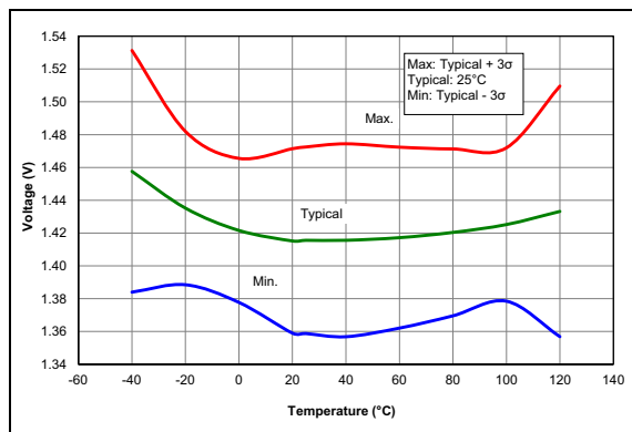
FIGURE 28-41: POR Rearm Voltage, PIC18F1XK50 Only.
