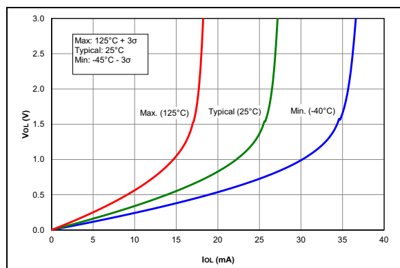
FIGURE 28-37: V_{OL} vs. I_{OL} , Over Temperature, V_{DD} = 3.0V .
