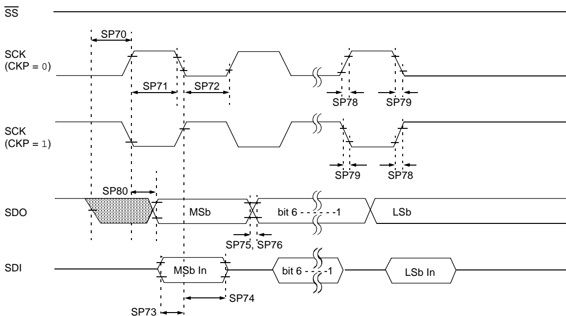
FIGURE 27-15: SPI MASTER MODE TIMING (CKE = 0, SMP = 0)
