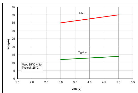
FIGURE 28-27: I_{PD} , Brown-out Reset (BOR), BORV = 1 , PIC18F1XK50 Only.
