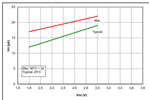
FIGURE 28-25: I_{PD} , Fixed Voltage Reference (FVR), PIC18LF1XK50 Only.
