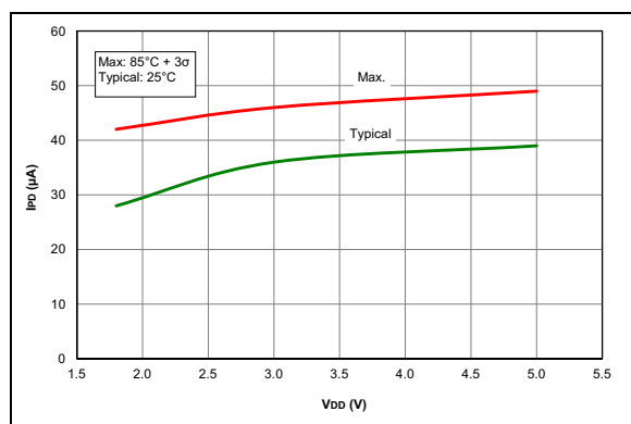
FIGURE 28-26: I_{PD} , Fixed Voltage Reference (FVR), PIC18F1XK50 Only.
