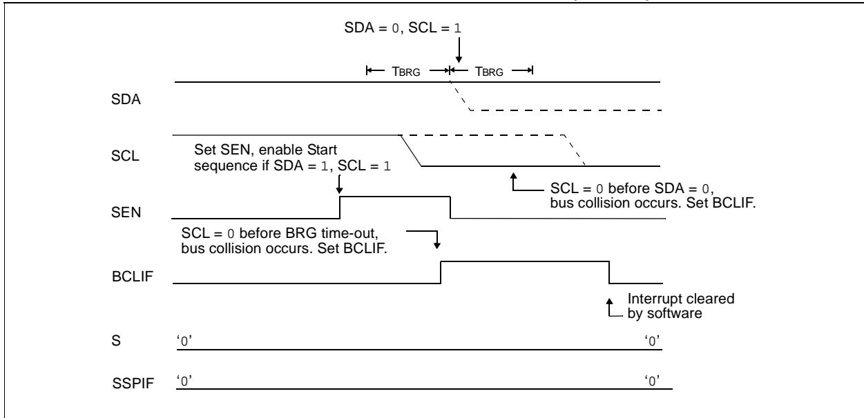
FIGURE 15-28: BRG RESET DUE TO SDA ARBITRATION DURING START CONDITION
