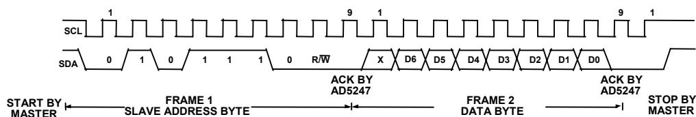
Figure 4. Writing to the RDAC Register
