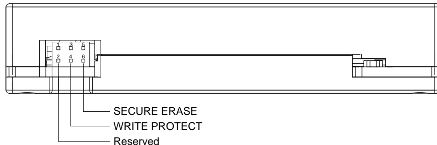
Figure 4: SSD Serial ATA 2.5" Write Protect Jumper Settings
