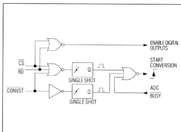
Figure 12. Conversion-Control Logic
