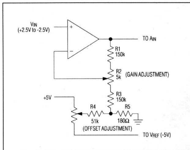
Figure 19. Offset and Gain Adjustment (Noninverting)
