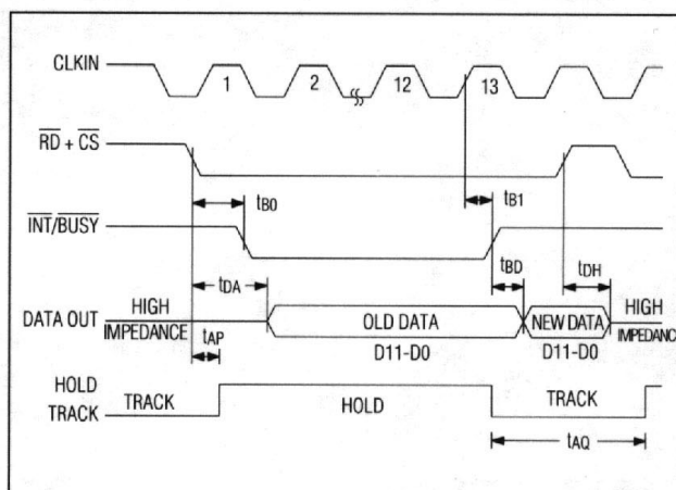
Figure 9. Slow-Memory Mode (Mode 3)
