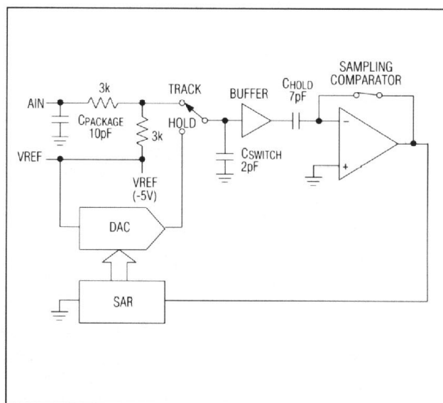
Figure 4. Equivalent Input Circuit
