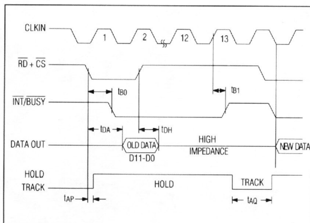
Figure 10. ROM Mode (Mode 4)
