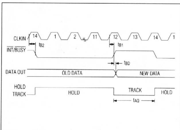
Figure 11. Continuous-Conversion Mode (Mode 5)
