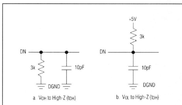
Figure 2. Load Circuits for Bus-Relinquish Time
