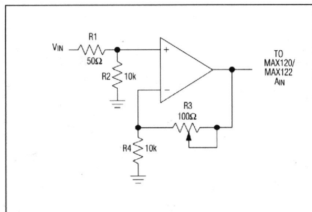
Figure 18. Trim Circuit for Gain Only
