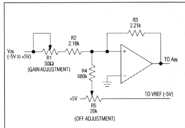
Figure 20. Offset and Gain Adjustment (Inverting)
