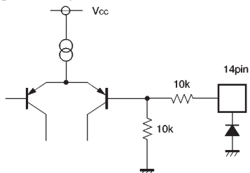
Regulator output
