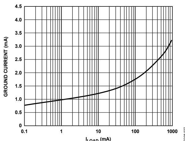
Figure 27. Ground Current vs. Load Current ( I_{LOAD} ), Adjustable Version, V_{OUT} = 1.2\text{ V}
