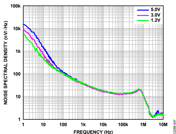
Figure 47. Output Noise Spectral Density, Different Output Voltages, Load Current = 100 mA
