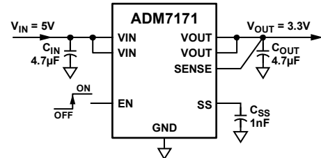
Figure 1. ADM7171 with Fixed Output Voltage, 3.3 V
