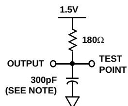
TELOV OUTPUT HIGH ENABLE LOAD CIRCUIT
