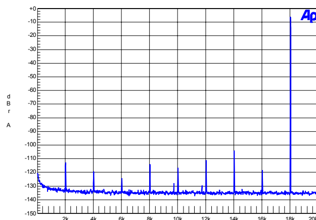
Figure 32. FFT (IMD 192 kHz)
