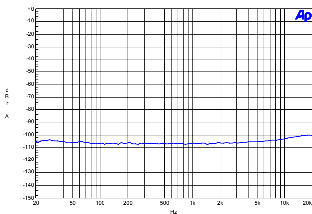
Figure 11. 48 kHz, Crosstalk
