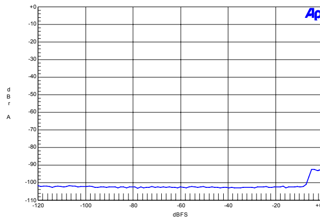
Figure 34. 192 kHz, THD+N vs. Level
