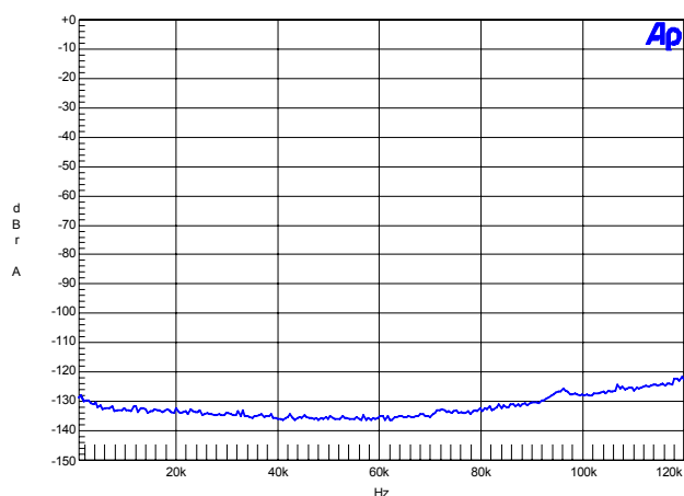
Figure 30. FFT (192 kHz Out-of-Band, No Input)
