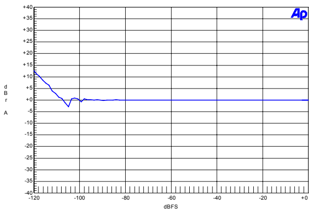
Figure 9. 48 kHz, Fade-to-Noise Linearity
