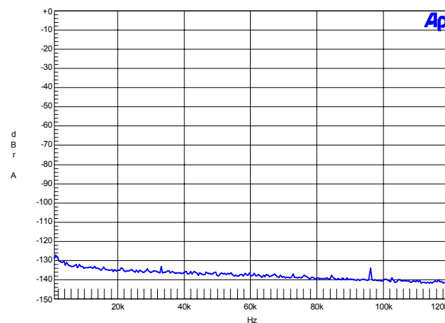
Figure 17. FFT (96 kHz Out-of-Band, No Input)
