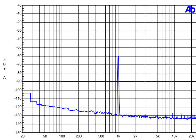
Figure 5. FFT (48 kHz, -60 dB Wideband)
