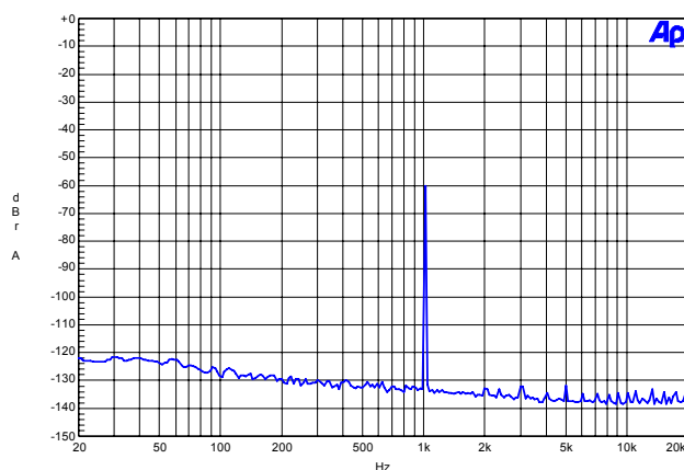
Figure 28. FFT (192 kHz, -60 dB)
