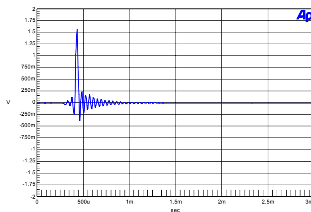
Figure 12. 48 kHz, Impulse Response
