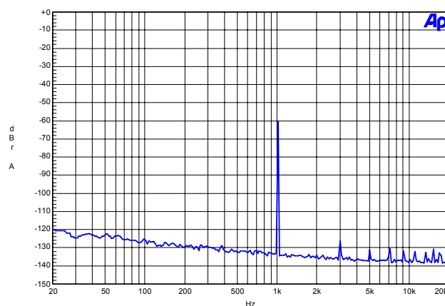
Figure 2. FFT (48 kHz, -60 dB)
