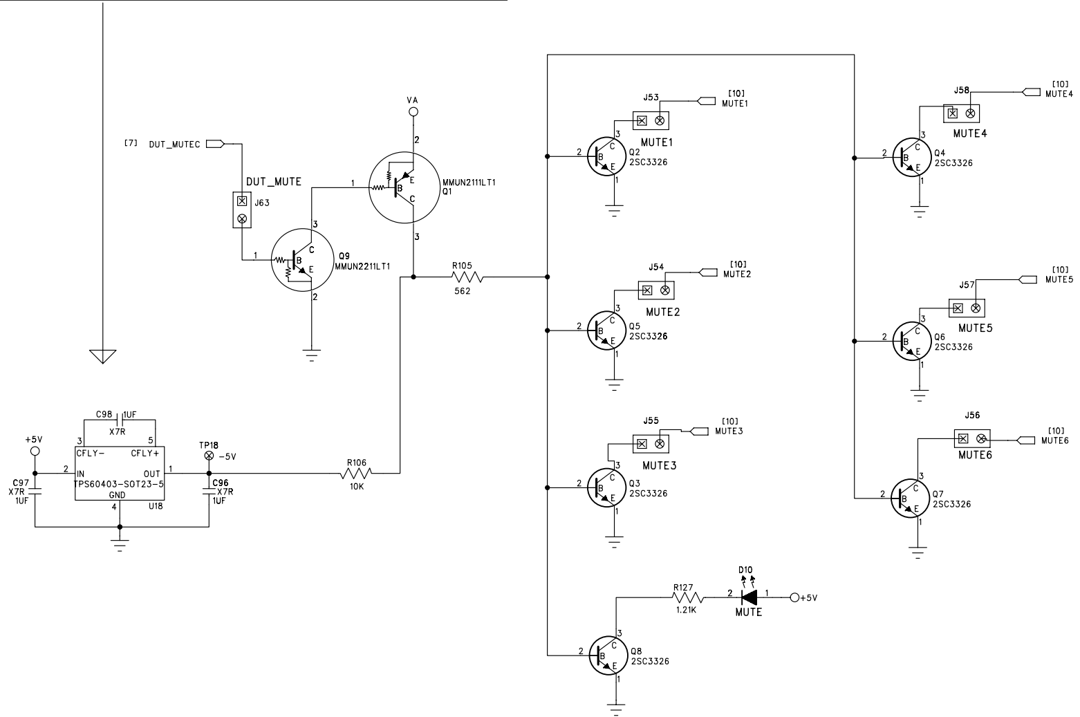
Figure 45. Mute Circuitry
