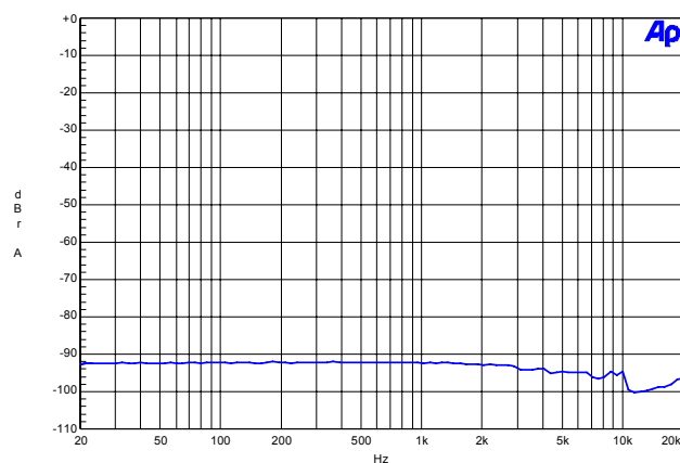
Figure 7. 48 kHz THD+N vs. Input Freq
