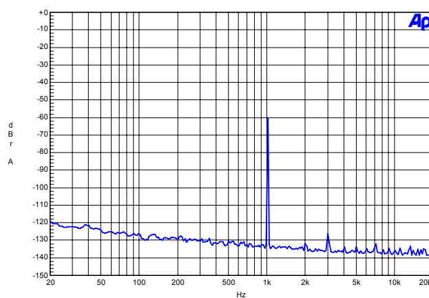
Figure 15. FFT (96 kHz, -60 dB)
