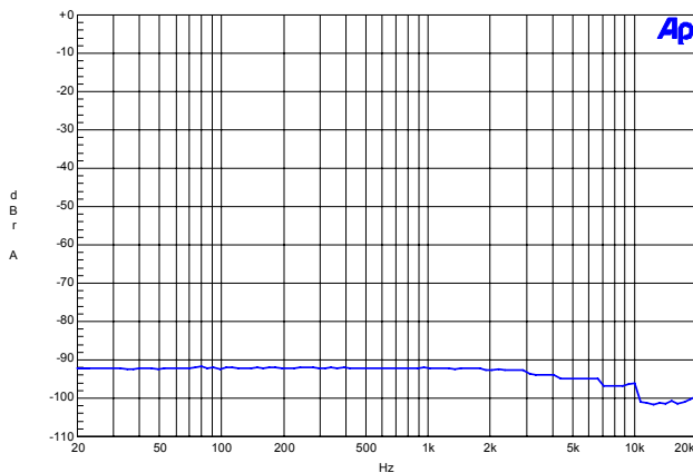
Figure 33. 192 kHz, THD+N vs. Input Freq
