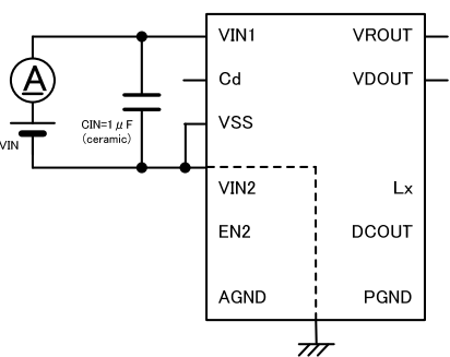
Circuit No.2
