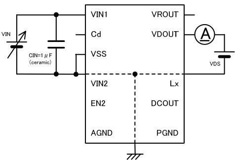
Circuit No.5
