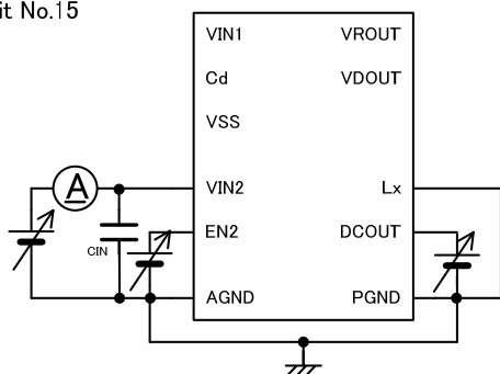
Circuit No.15
