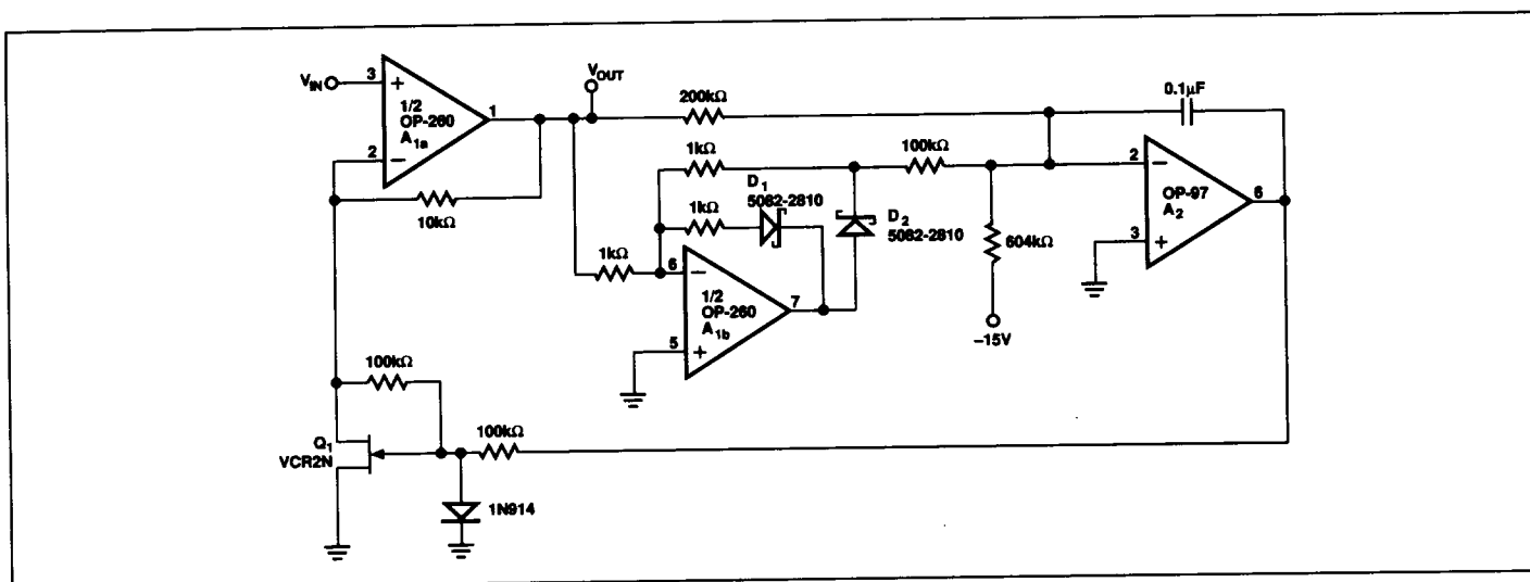
FIGURE 12: The OP-260 eliminates the problem of variable bandwidth in AGC amplifiers using voltage feedback op amps.
