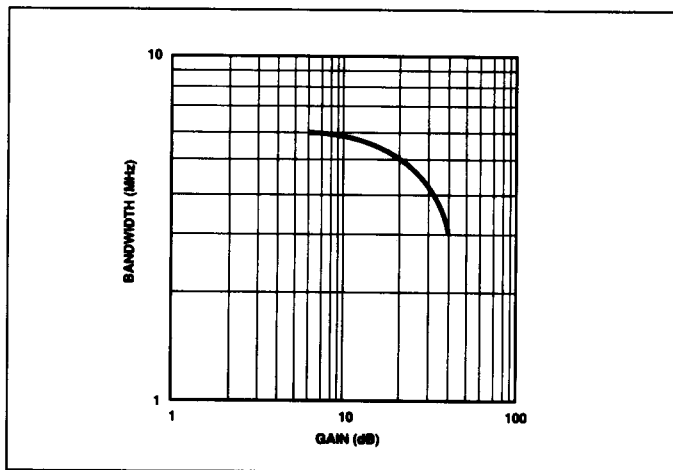
FIGURE 17: Bandwidth versus gain for the high speed instrumentation amplifier.
