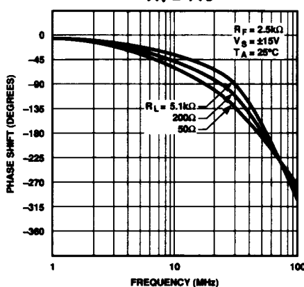
PHASE SHIFT vs FREQUENCY A_V = +10
