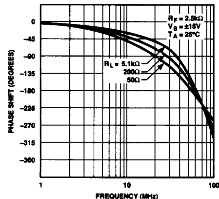
PHASE SHIFT vs FREQUENCY A_V = +5
