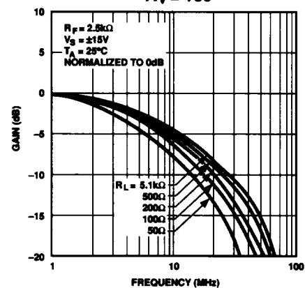
GAIN vs FREQUENCY A_V = +50
