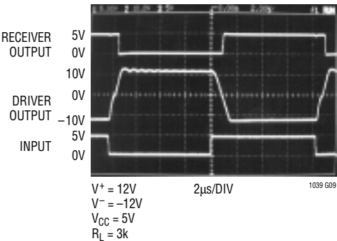
Output Waveforms
