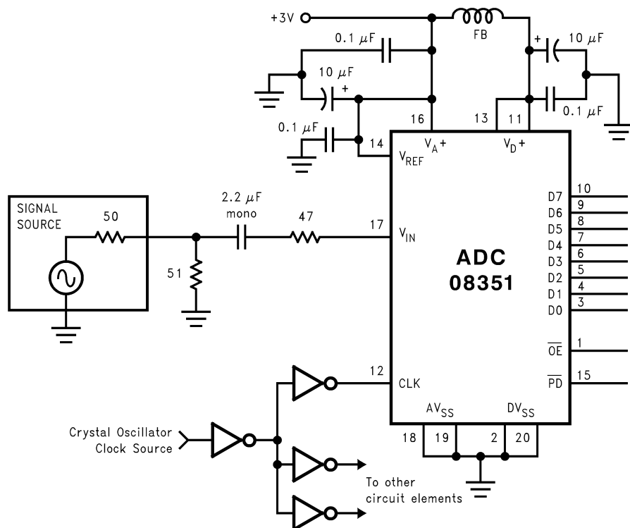
Figure 23. AC Coupled Circuit for a Low Impedance Source Located Near the Converter
