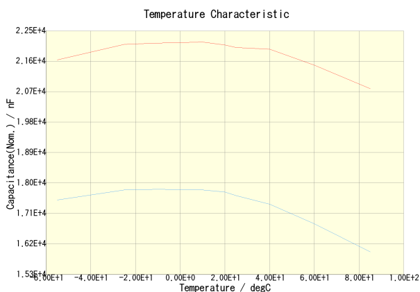
C3225X5R1C226K250AA(DC Bias = 0V) C3225X5R1C226K250AA(DC Bias = 8V)
