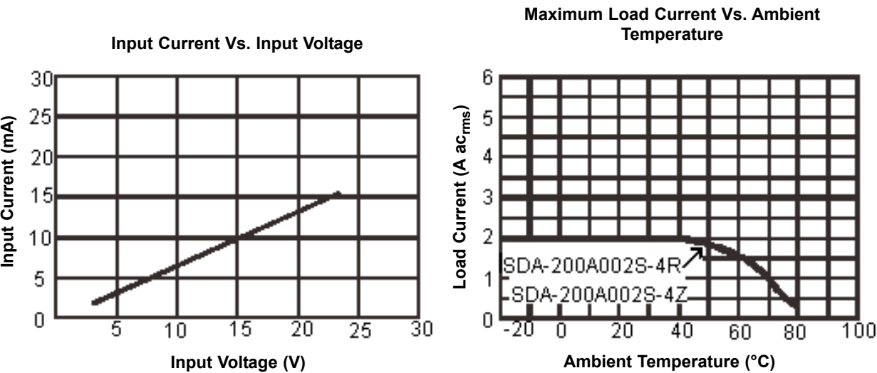
Characteristic Curves
