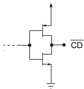
Figure 5-5: \overline{CD} Circuit
