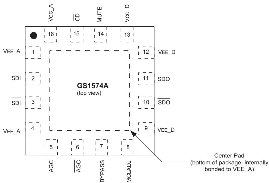
Figure 1-1: 16-Pin QFN
