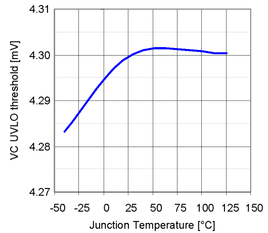
Figure 8: VC UVLO threshold vs. temperature
