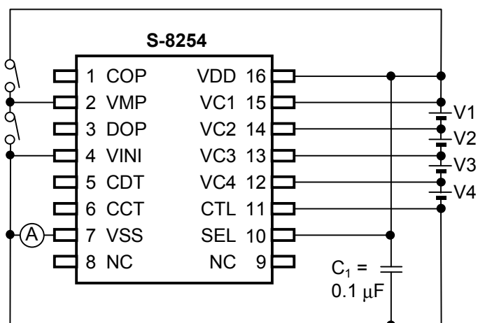
Test Circuit 1
