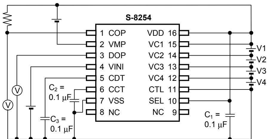
Test Circuit 3
