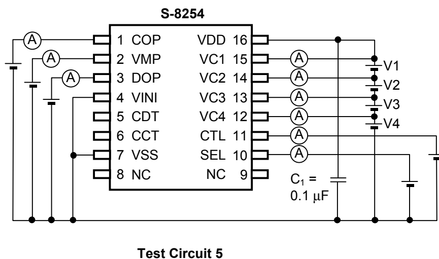
Figure 3 Test Circuit (2/2)
