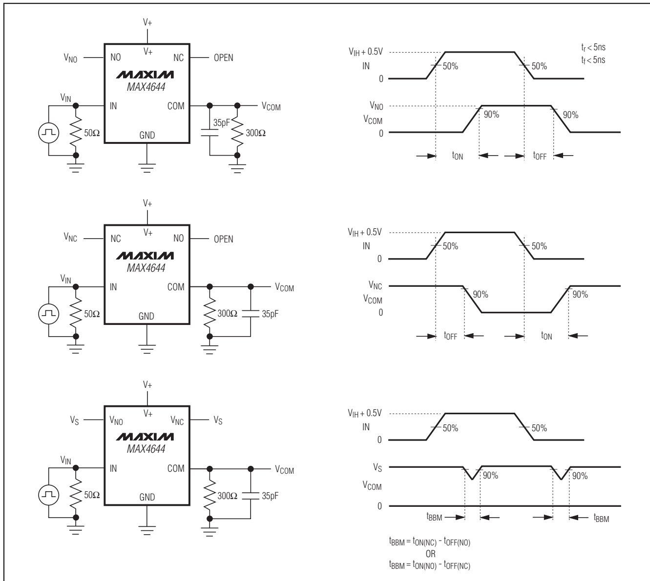
Figure 2. Switching Times
