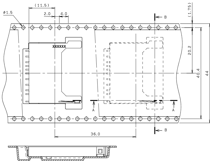
SECT. A-A
