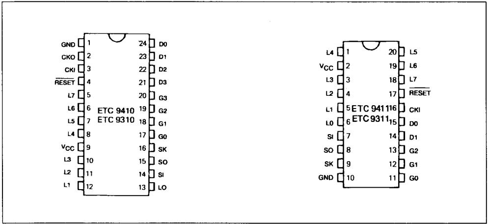
Figure 2 : Pin Connections.
