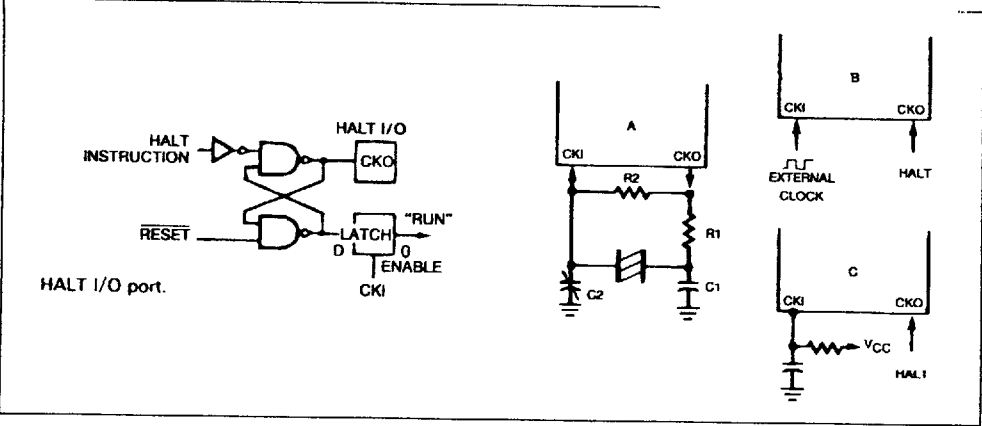
Figure 6 : ETC9410C Oscillator.
