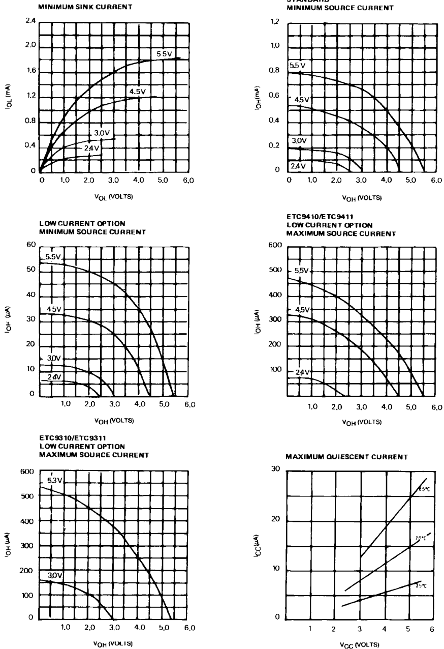
Figure 8 : Input/output Characteristics.
