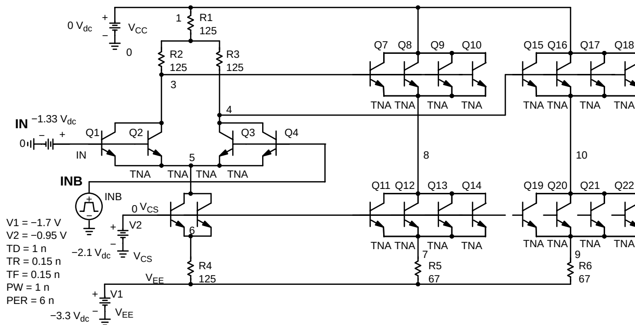
Figure 3. Typical INBUF
