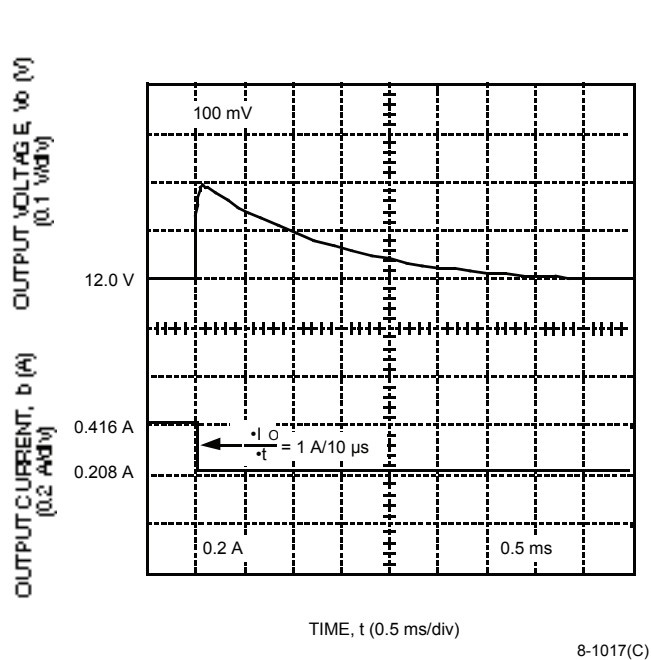
Figure 5. CC025 Dual-Output-Series Typical 12 V Output Voltage Response to a Step Load Change from 50% to 25% of I_{o,max} at V_i = V_{i,nom} and T_c = 25\text{ }^{\circ}\text{C}
