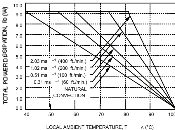
Figure 19. Total Power Dissipation vs. Local Ambient Temperature and Air Velocity
