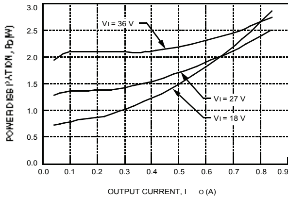
Figure 18. 15 V Output Power Dissipation vs. Output Current
