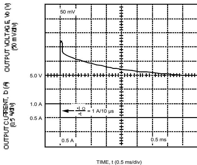
Figure 4. CC025 Dual-Output-Series Typical 5 V Output Voltage Response to a Step Load Change from 50% to 25% of I_{o, \text{max}} at V_i = V_{i, \text{nom}} and T_c = 25^\circ\text{C}
