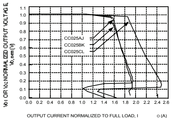
Figure 2. CC025 Dual-Output-Series Normalized Output Current vs. Normalized Output Voltage at V_i = 28\text{ V} and T_c = 25^\circ\text{C}
