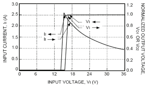
Figure 1. CC025 Dual-Output-Series Input Current and Normalized Output Voltage vs. Input Voltage at Full Load and T_c = 25^\circ\text{C}
