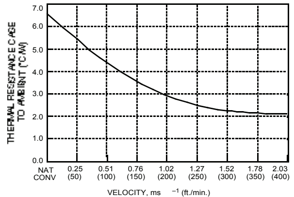
Figure 20. Case-to-Ambient Thermal Resistance vs. Air Velocity
