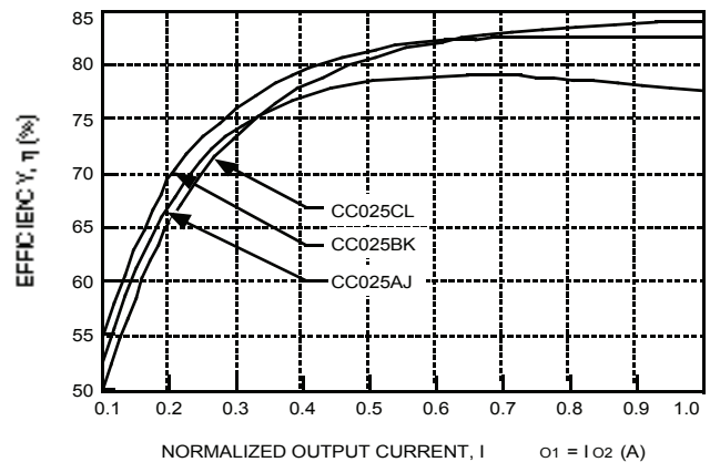
Figure 3. CC025 Dual-Output-Series Efficiency vs. Normalized Output Currents at V_i = 28\text{ V} and T_c = 25^\circ\text{C}
