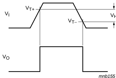
Fig 8. Definition of V_{T+} , V_{T-} and V_H
