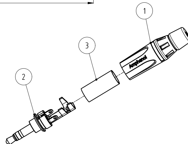
EXPLORED VIEW ( 1 : 1 )
