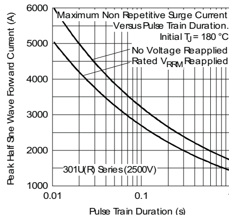
Fig. 11 - Maximum Non-Repetitive Surge Current
