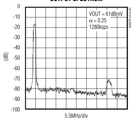
OUTPUT SPECTRUM
