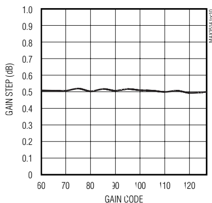
GAIN STEP vs. GAIN CODE HIGH-POWER MODE
