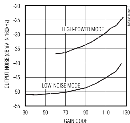
TRANSMIT NOISE vs. GAIN CODE
