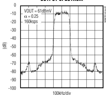
OUTPUT SPECTRUM
