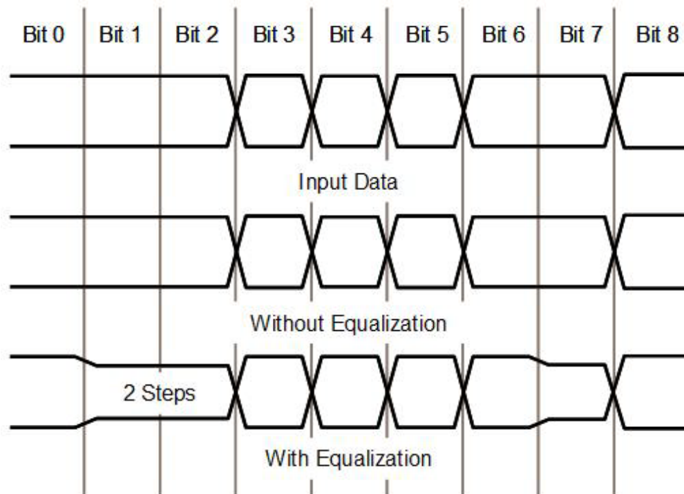
Figure 6. Driver Equalization
