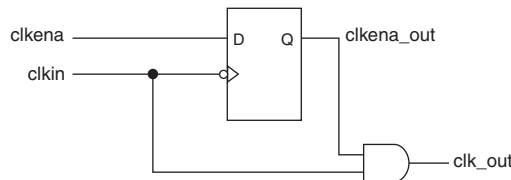
Figure 5-7. clkena Implementation
