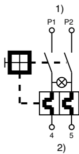
2-pole thermal protected, illuminated
