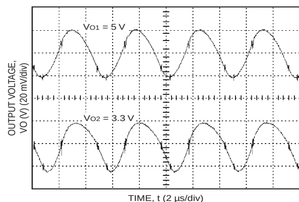
Figure 2. Typical Output Ripple and Noise.
