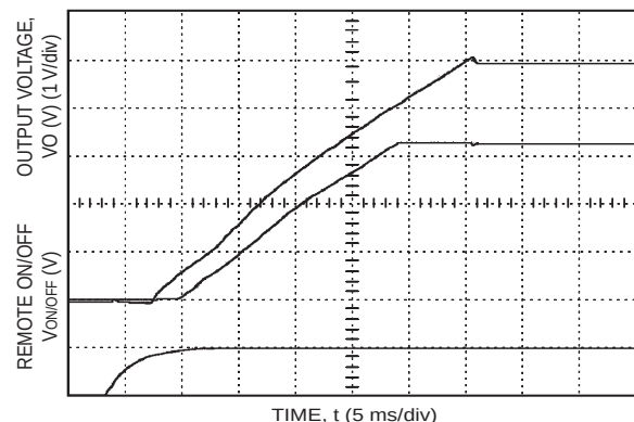
Figure 1. Typical Start-Up Using Remote On/Off.
