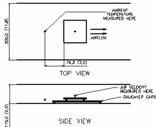
Figure 22.Thermal Test Setup
