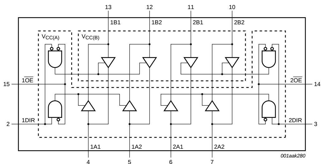
Fig 1. Logic symbol
