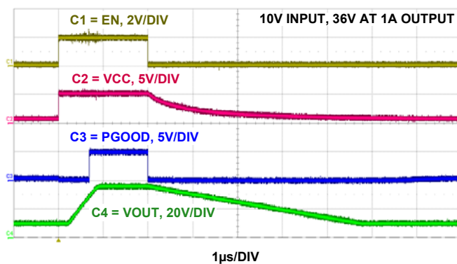
FIGURE 11. ENABLE/DISABLE WAVEFORMS
