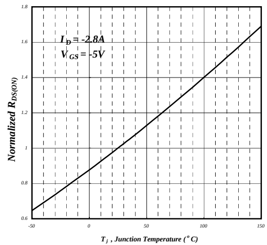
Fig 4. Normalized On-Resistance
