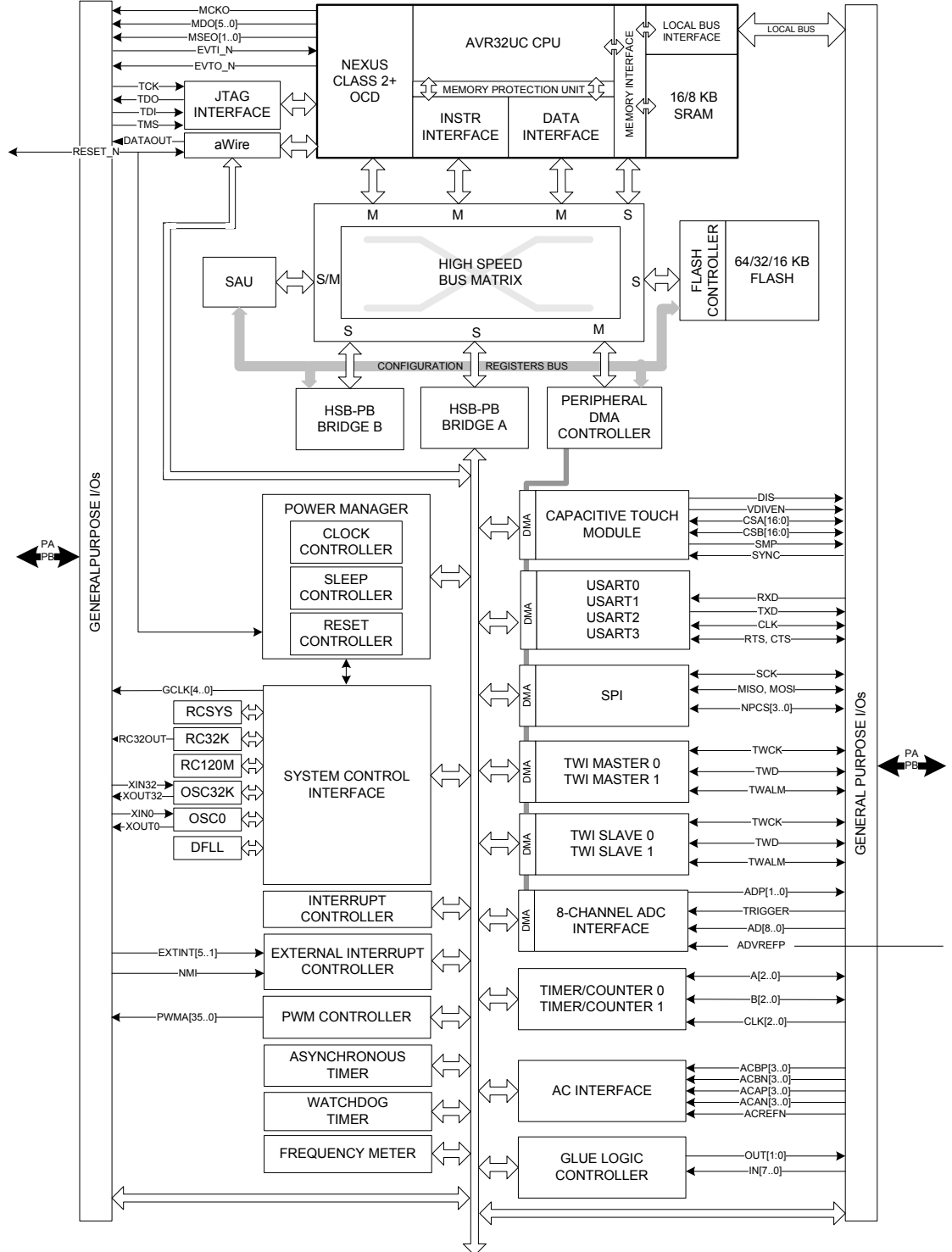
Figure 2-1. Block Diagram
