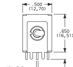
Actuator Shown In Pos. 1 .125 TYP. (3,18) Terminals & Support
