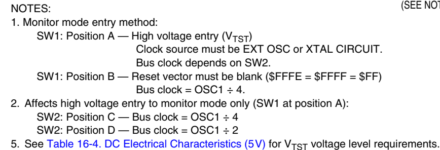
Figure 7-1. Monitor Mode Circuit
