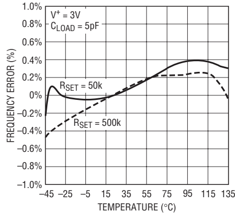
Typical Frequency Error vs Temperature
