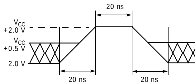
Figure 17.1 Maximum Overshoot Waveforms
