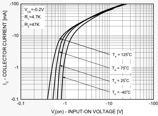
Figure 3. Input-On Voltage
