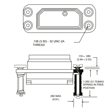
Mounting Style K With Captive Springs
