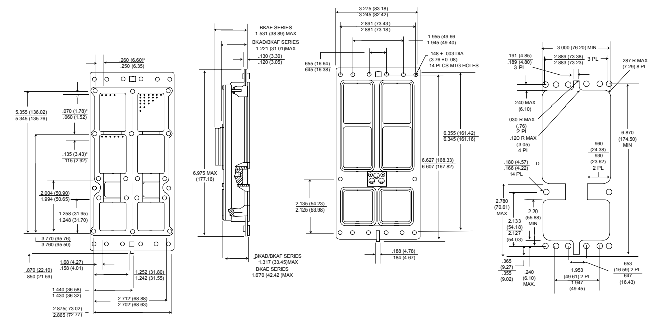
Retainer Plate
