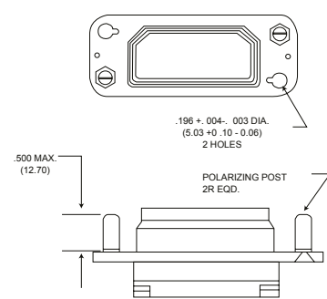
Mounting Style A
