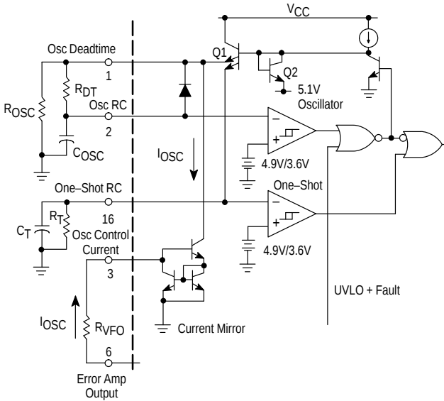
Figure 2. Oscillator and One-Shot Timer
