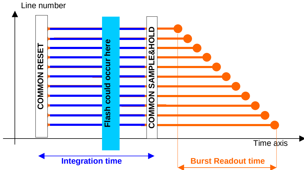
Figure 14. Synchronous Shutter Operation
