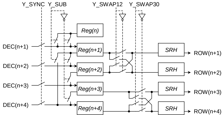
Figure 7. Row Structure
