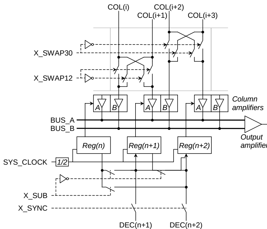
Figure 6. Column Structure
