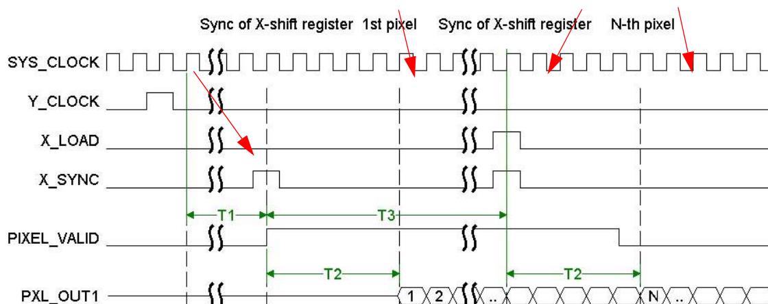
Figure 23. Pixel Output
