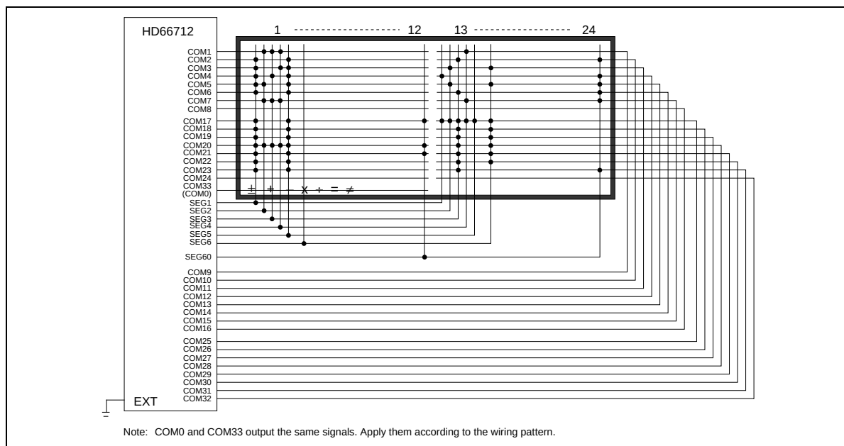
Figure 26 24 x 1-Line + 60-Segment Display (5-Dot Font, 1/33 Duty)
