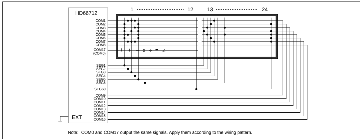
Figure 25 24 x 1-Line + 60-Segment Display (5-Dot Font, 1/17 Duty)
