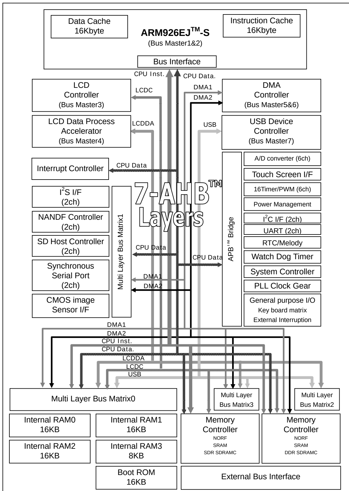
Figure 1.1 TMPA910CRA block diagram
