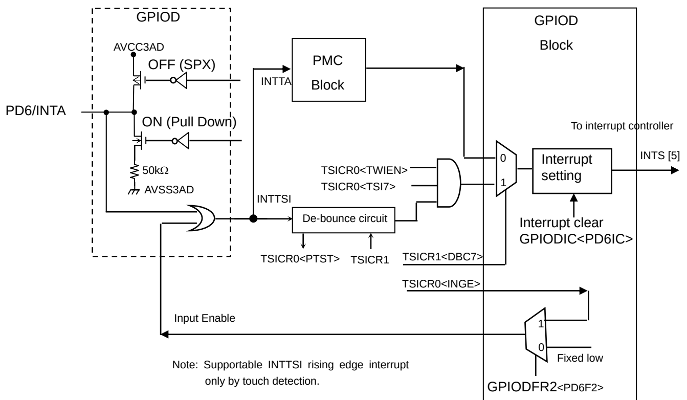
Figure 3.21.3 Block diagram of touch detection
