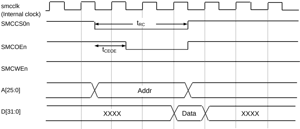
Figure 3.10.18 Asynchronous Read
