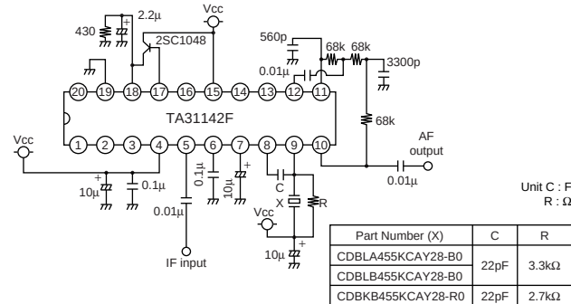
TA31142
