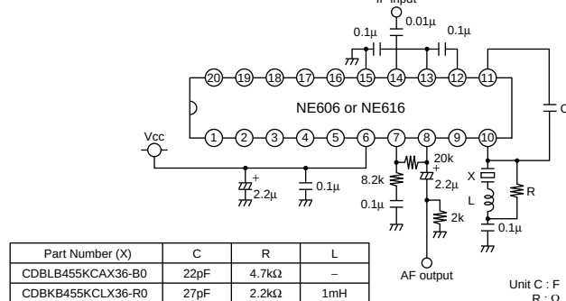
NE(SA)606/616
