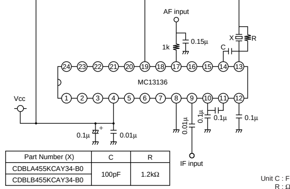
MC13136
