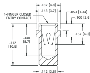
.065 (1.65) - .082 (2.08) PIN - SOLDER MOUNT
