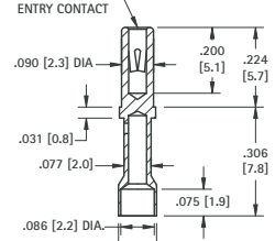
.032 (.81) - .046 (1.17) PIN - CRIMP BARREL JACK
