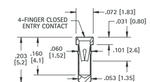
IC SOCKET CONTACTS FOR .015 (.38) - .025 (.64) LEADS - PRESS-FIT
