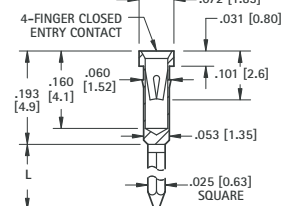
IC SOCKET CONTACTS FOR .015 (.38) - .025 (.64) LEADS - PRESS-FIT
