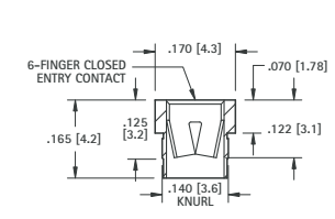
.084 (2.13) - .102 (2.6) PIN - PRESS-FIT
